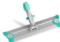
Aluminium mop holder and anti-bacterial plastic components with strips for strap tape system and Lock System fitting
